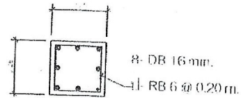
Detail C
