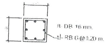
Detail C
